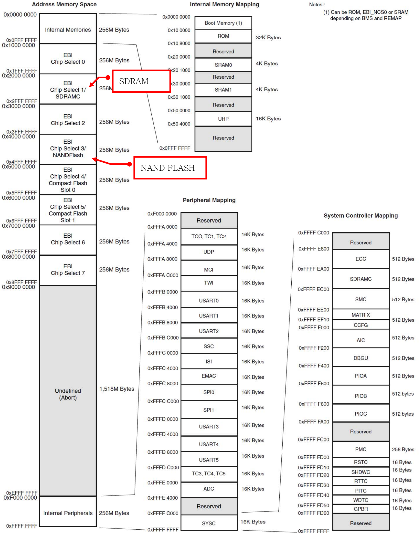
Figure 8-1. AT91SAM9260 Memory Mapping
